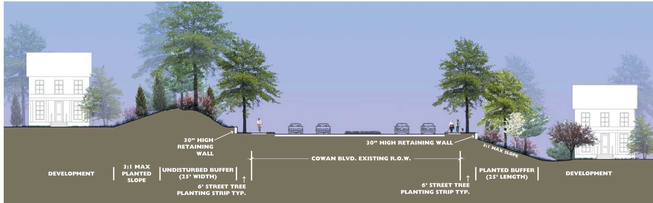
COWAN BOULEVARD - STREET TREE RETROFIT PROPOSED SECTION / ELEVATION (LOOKING NORTHWEST)
